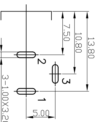
Pin Hole Layout (Jack Bottom View)
