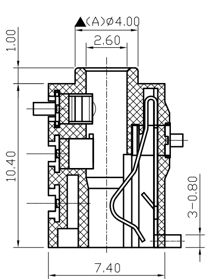
SEC: C-C
