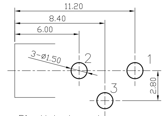
Pin Hole Layout (Jack Bottom View)
