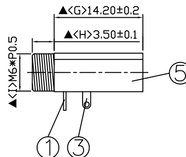
WITH THREAD
