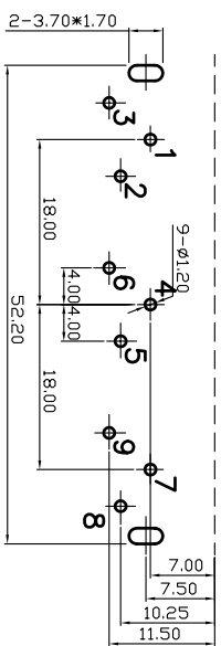
Pin Hole Layout (Jack Bottom View)
