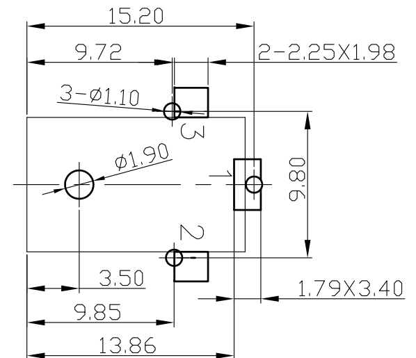
Pin Hole Layout (Jack Bottom View)
